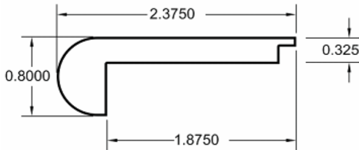
Stair Nosing
