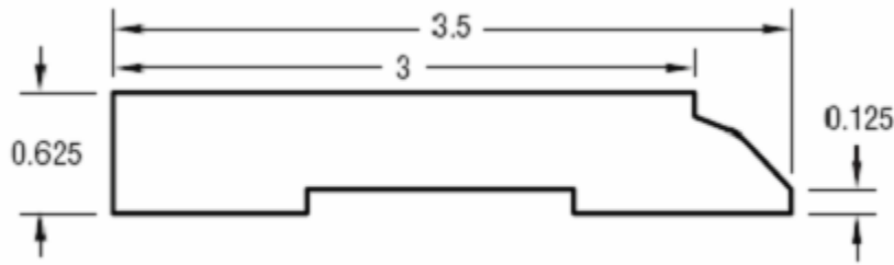
Wall Base
